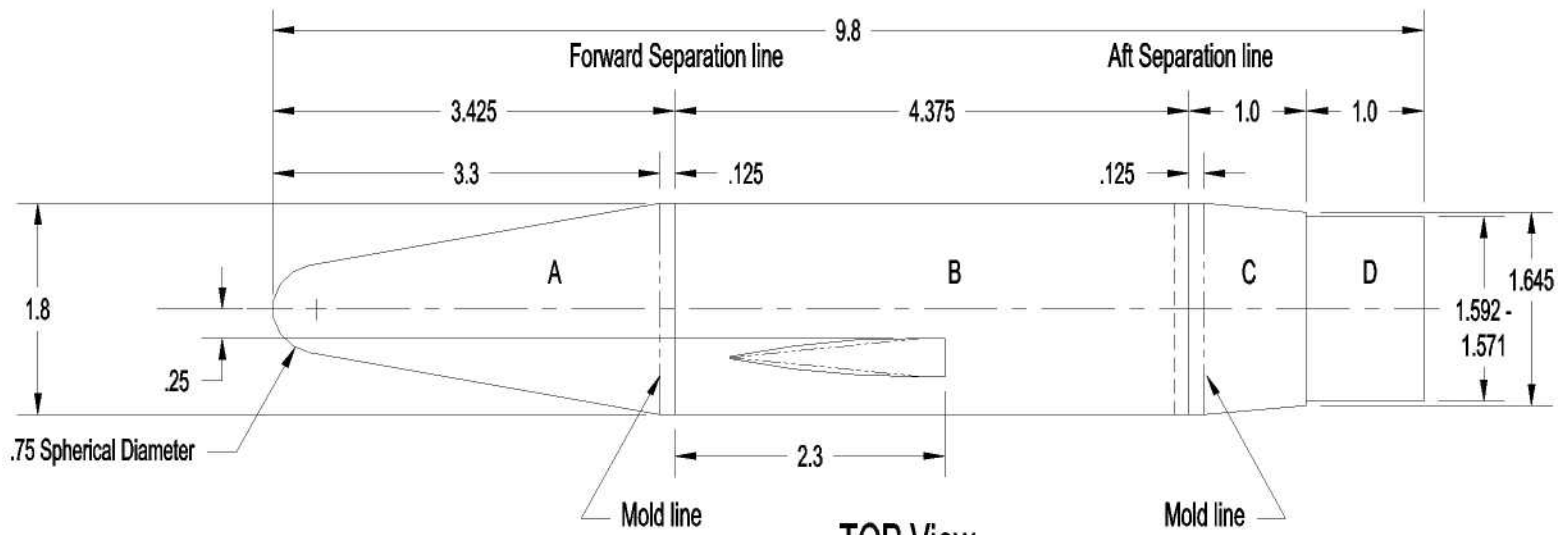
TOP View
